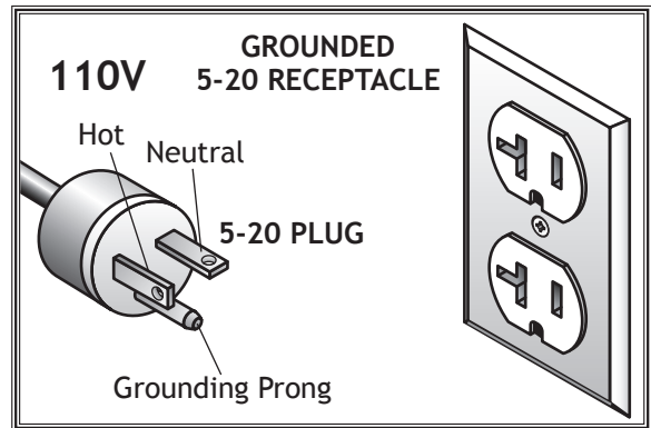
Figure 9. NEMA 5-20 plug & receptacle.
